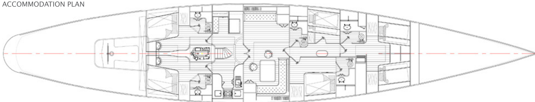
ACCOMMODATION PLAN
